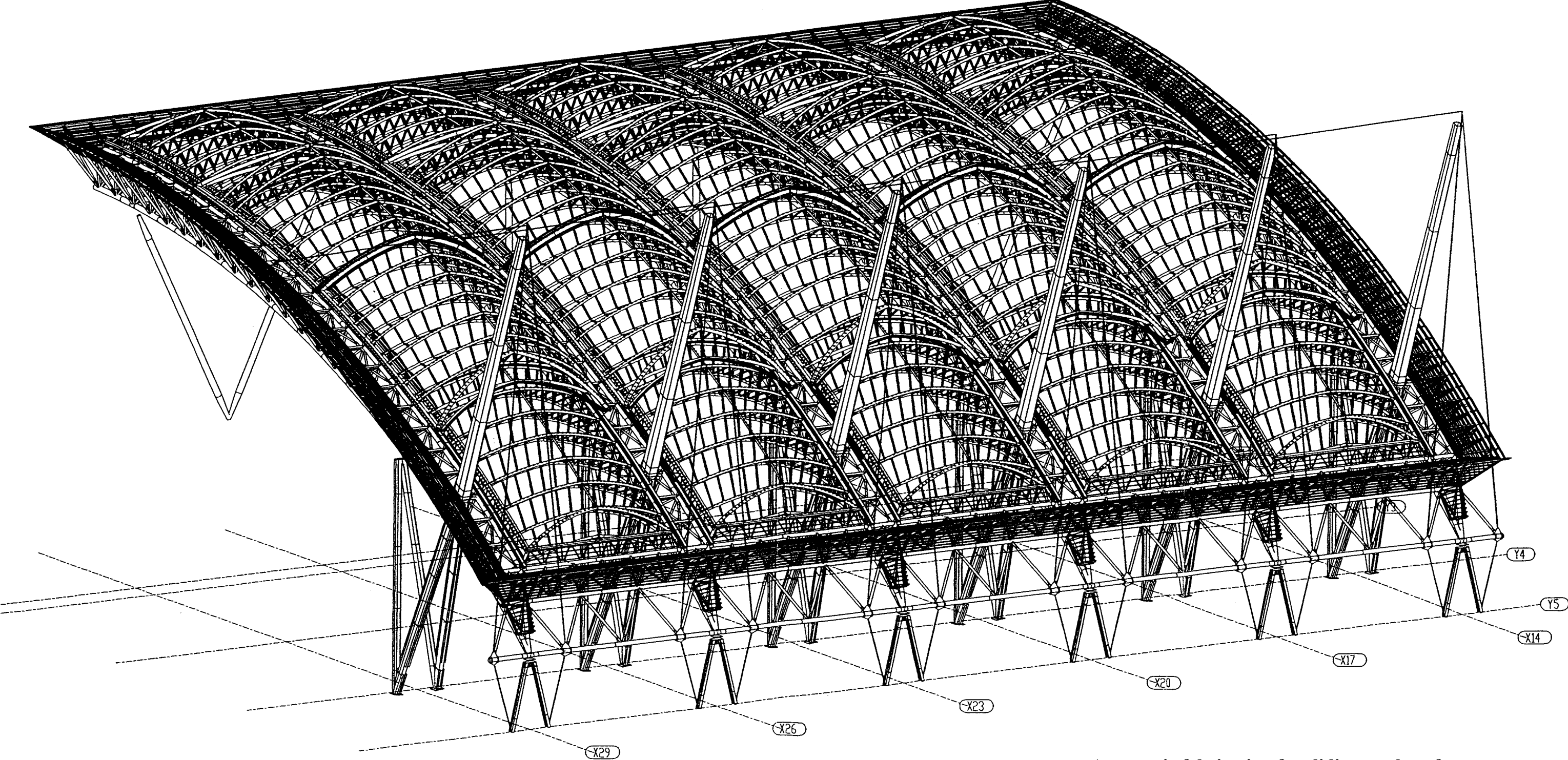
Automatic fabrication for sliding steel roof structure of Race track at Hong Kong with TEKLA Structure.
