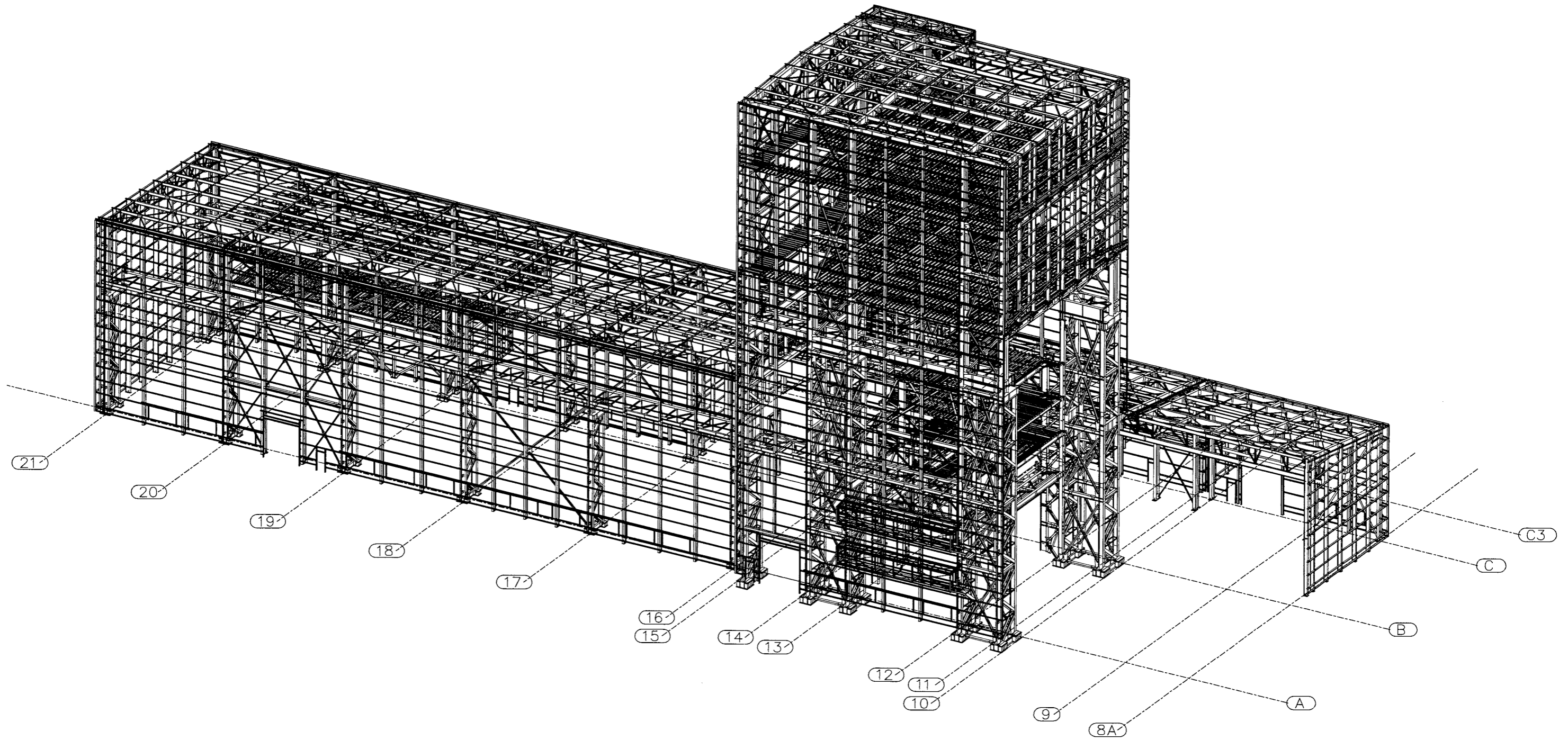
PERSPECTIVE VIEW
